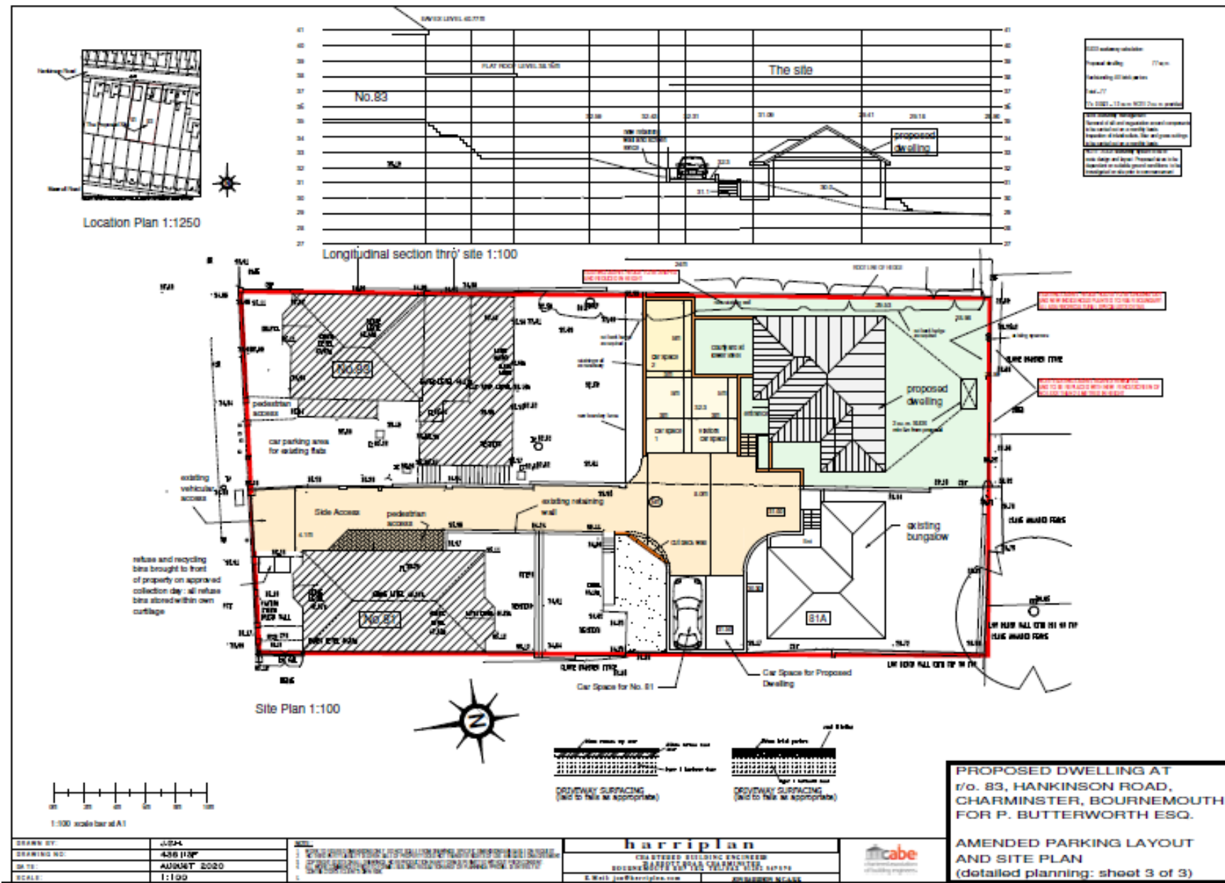
PROPOSED SITE PLAN (AMENDED – Drawing No:4381(3F))
