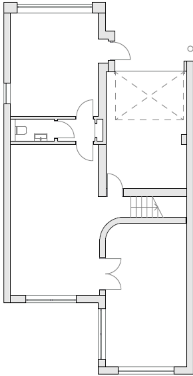
Existing Ground Plan Scale (A1): 1:100
