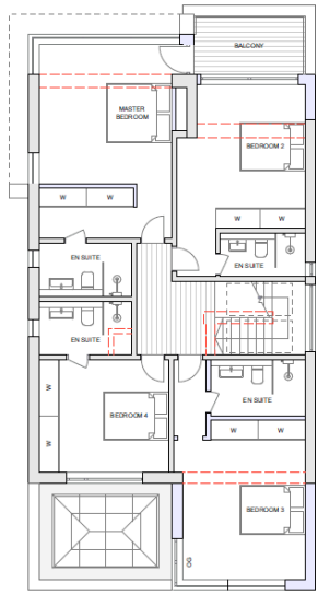
Proposed First Plan Scale (A1): 1:100
