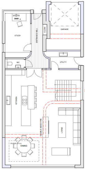
Proposed Ground Plan Scale (A1): 1:100
