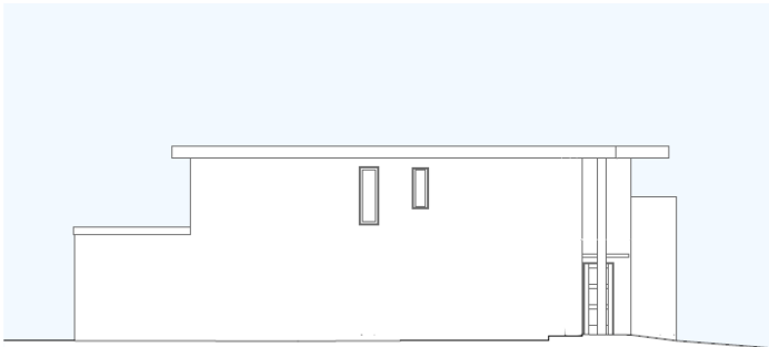
Existing Side Elevation Scale (A1): 1:100
