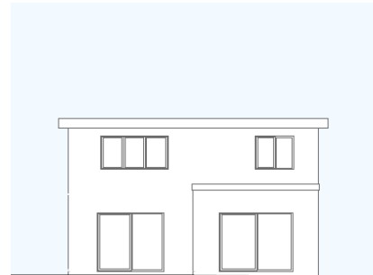
Existing Rear Elevation Scale (A1): 1:100
