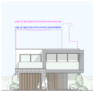
Proposed Front Elevation Scale (A1): 1:100
