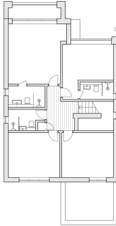
Existing First Plan Scale (A1): 1:100
