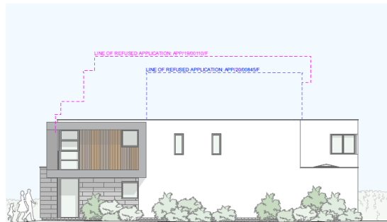
Proposed Side Elevation Scale (A1): 1:100
