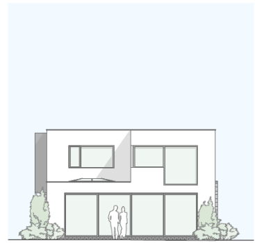
Proposed Rear Elevation Scale (A1): 1:100
