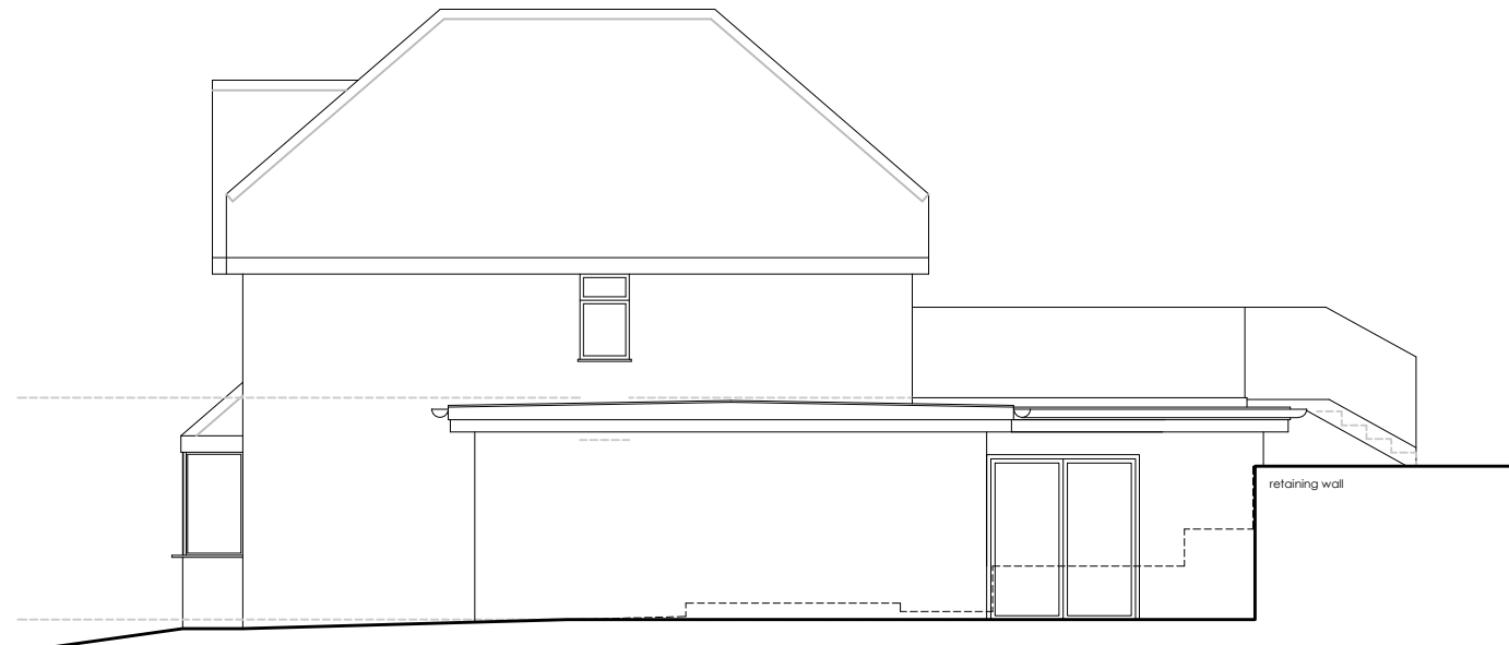
West Elevation
