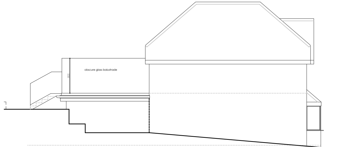
East Elevation
