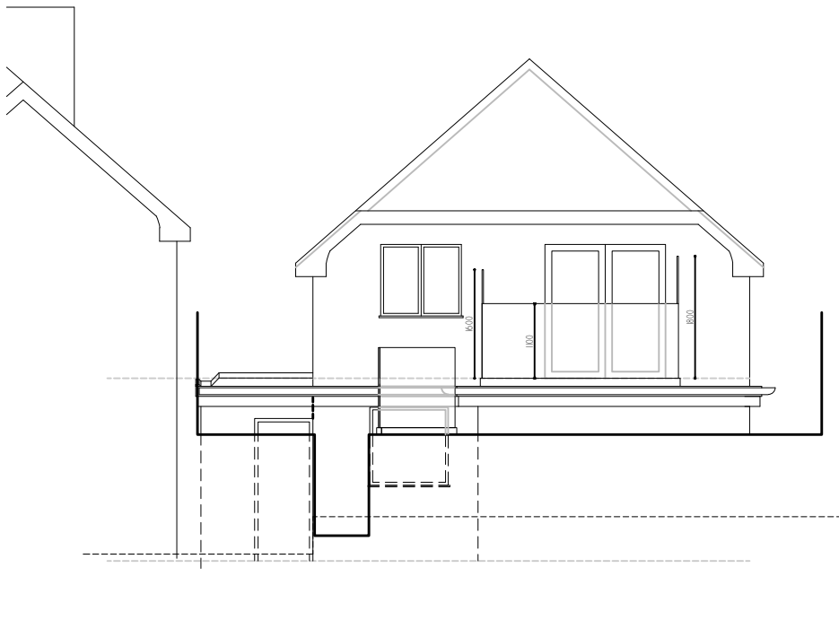
South Elevation
