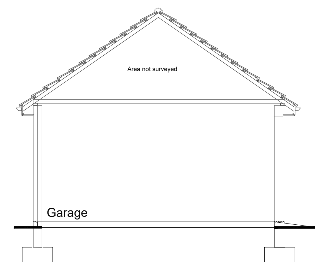
Section B-B 1:50
