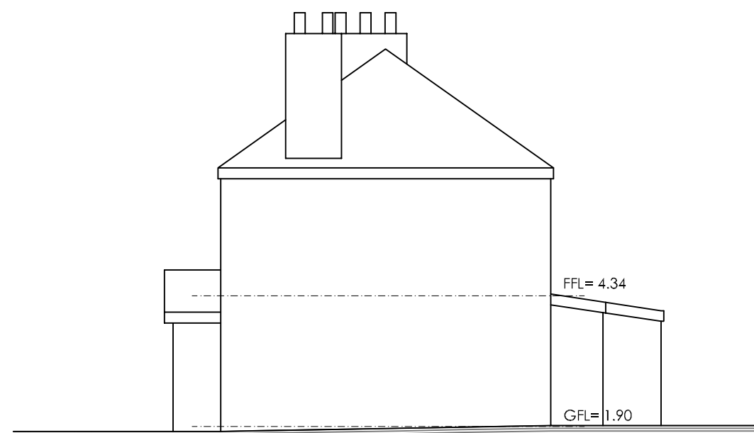
Side (North East) Elevation
