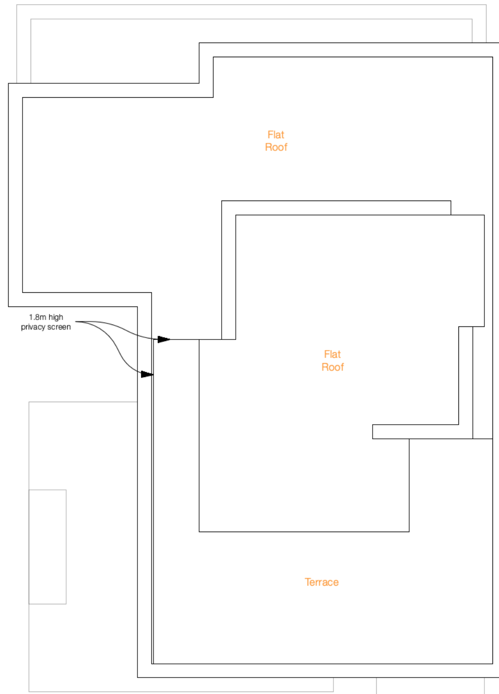
Roof Plan Scale 1:100 @A3
