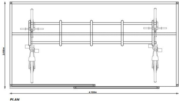
TYPICAL OXFORD CYCLE SHELTER
