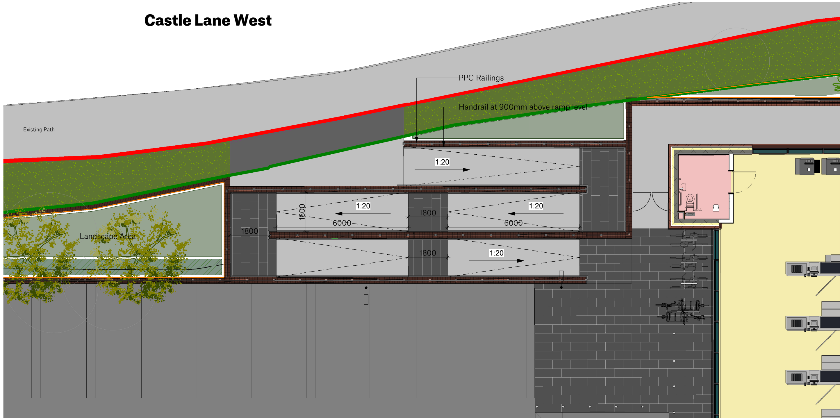
Proposed External Ramp 1:100
